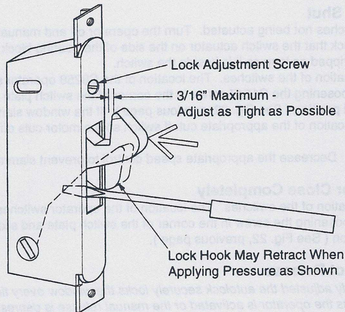
Fig. 24 - Adams Rite® MS1847-06 Hook-Type Lock Adjustments
