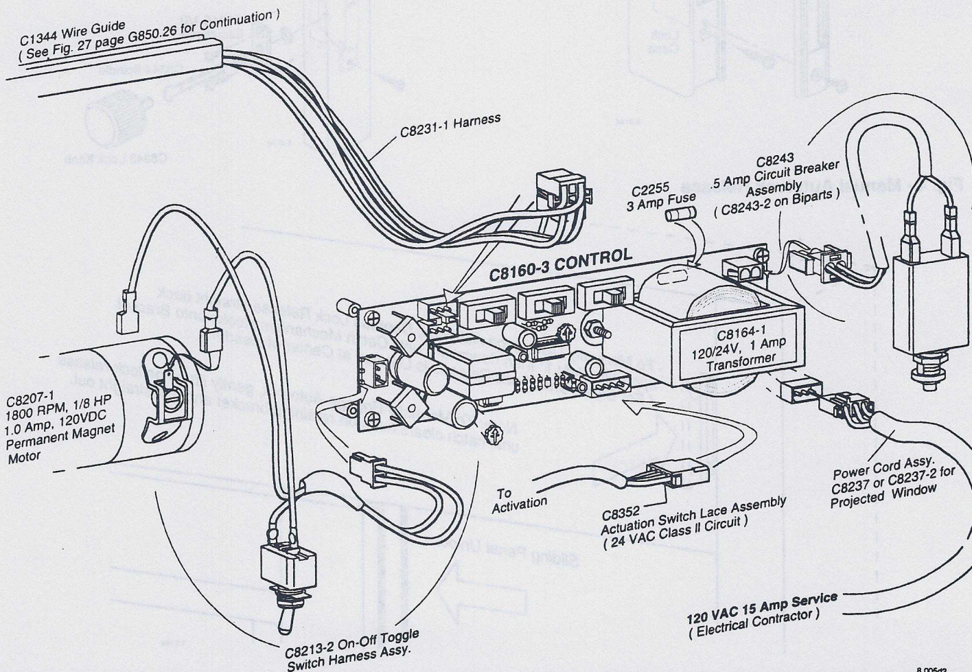
Fig. 5 - C8160-3 Master Control and Connections
