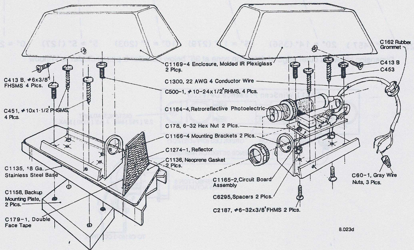
Fig. 14 - Exploded View of C1160-4
