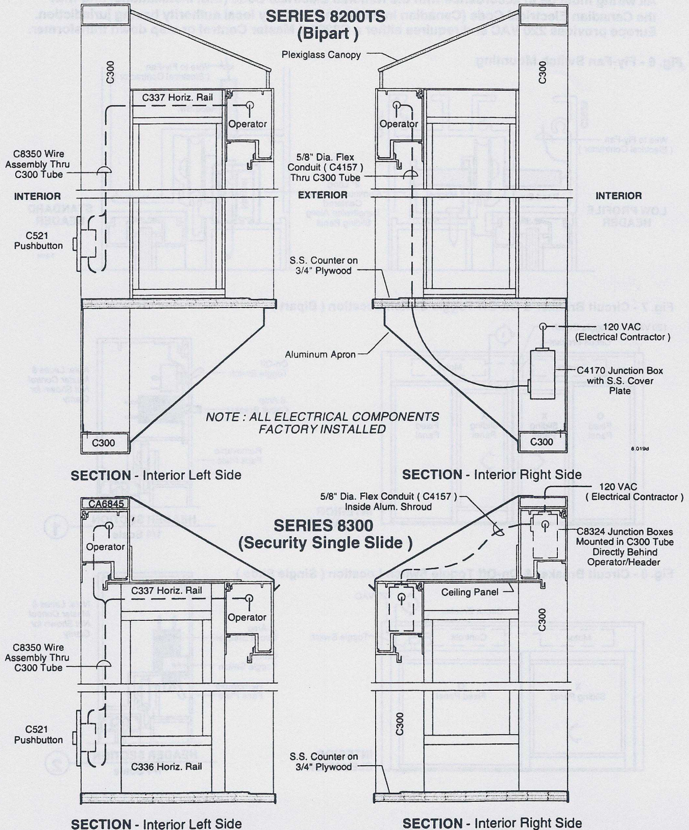
Fig. 9 - Projected Windows - Electrical Routing to Pushbuttons & Junction Boxes
