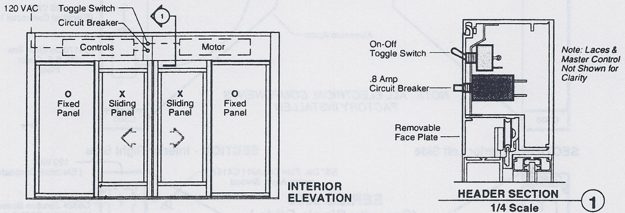
Fig. 7 - Circuit Breaker & On-Off Toggle Switch Location ( Bipart )
